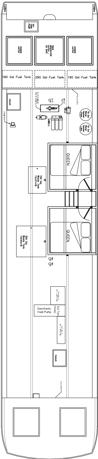
CUDDY FLOOR PLAN
