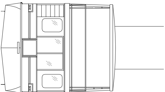
BOW ELEVATION
