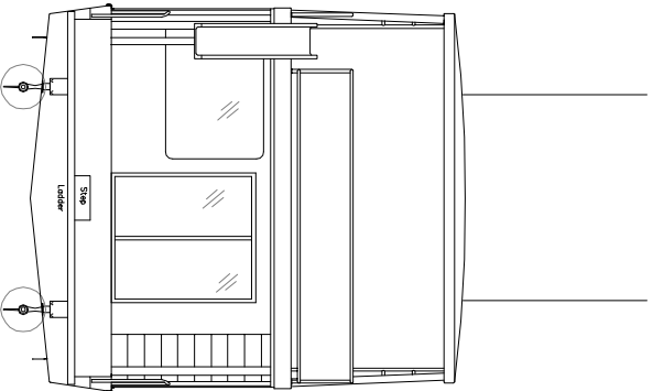
STERN ELEVATION
