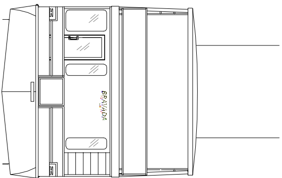
BOW ELEVATION
