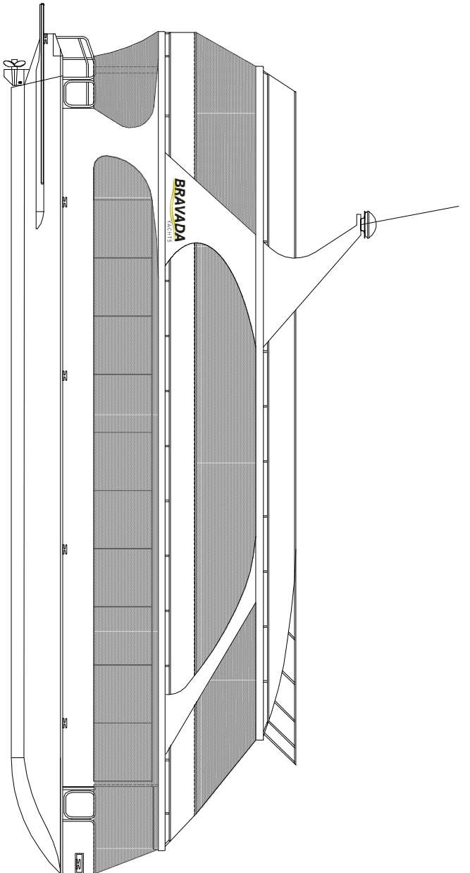
STARBOARD SIDE ELEVATION
