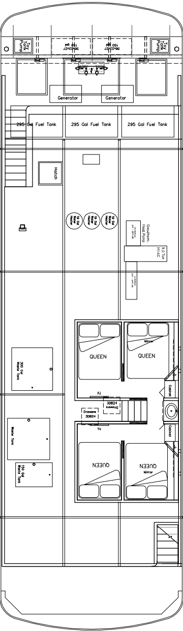
CUDDY FLOOR PLAN
