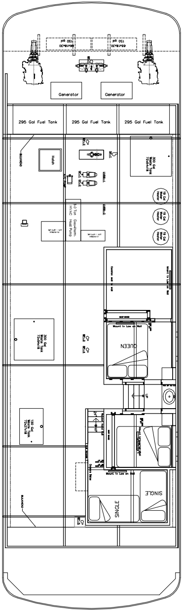
CUDDY FLOOR PLAN
