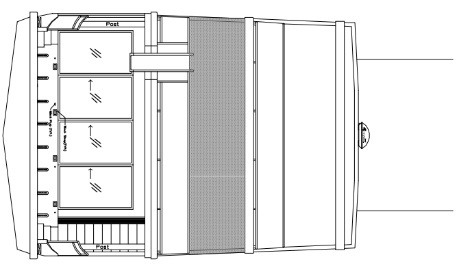
STERN ELEVATION
